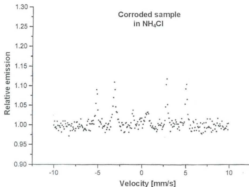
Figure 10. CEMS spectrum of corroded sample in a 5 \times 10^{-3} M \text{NH}_4\text{Cl} solution.
