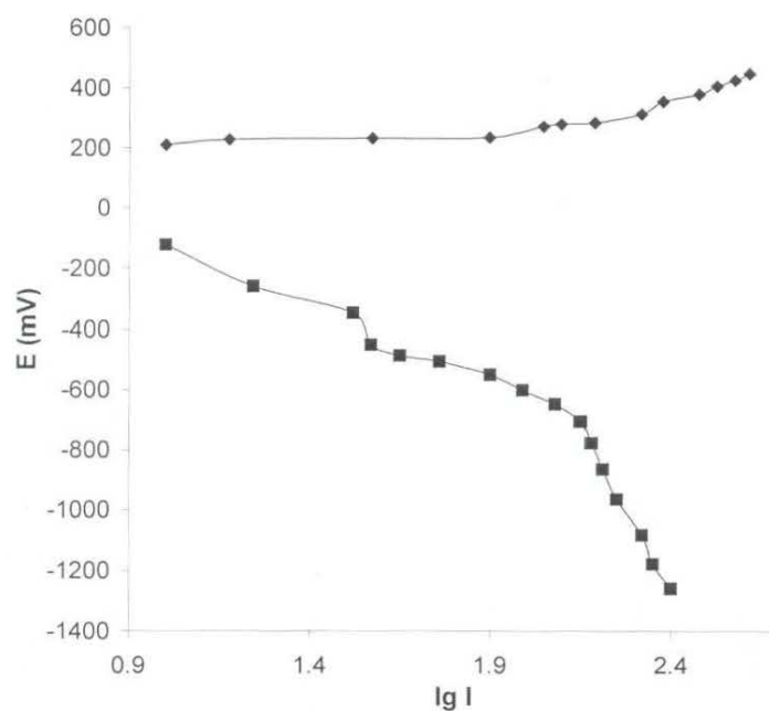
Figure 4. The anodic and cathodic polarization curves for carbon steel in ammoniacal solution containing 10^{-3} N \text{NH}_3 and 10^{-3} M \text{NH}_4\text{Cl} .
